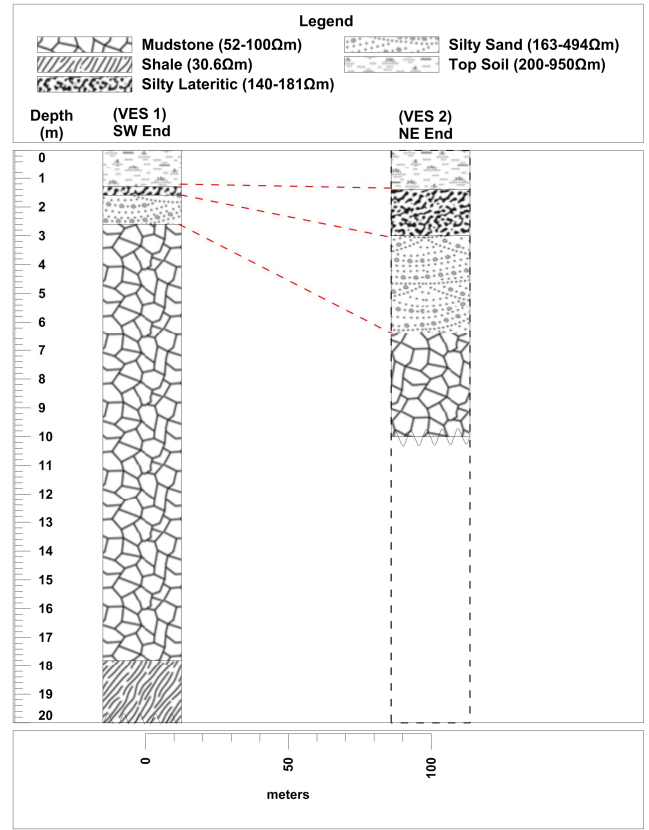
Figure 5. Geoelectric Section across VES points at Idembia bridge site.
