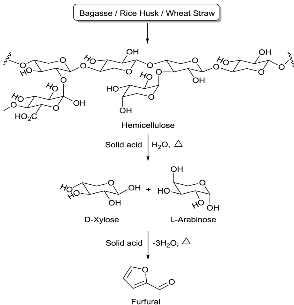
Fig. 1: One-Pot Conversion of Hemicellulose to Furfural, Using a Solid Acid Catalyst. Source: (Bhaumik and Dhepe 2014)
